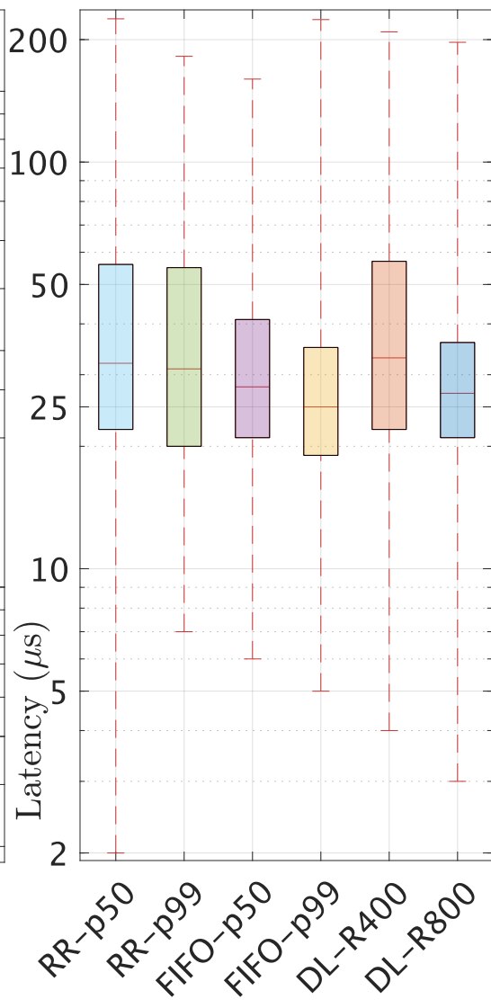
RT Schedulers - Stress
