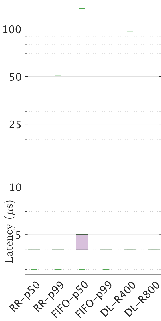
RT Schedulers - No Stress
